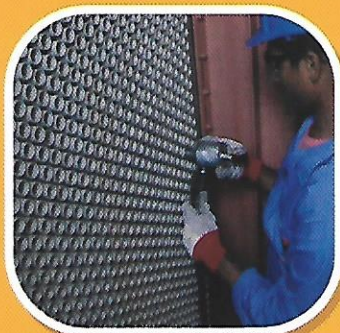
Tube Testing
